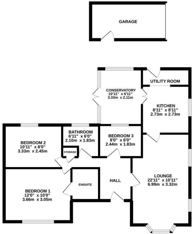
GROUND FLOOR 867 sq.ft. (80.5 sq.m.) approx.
